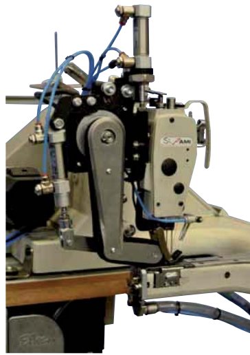
Patented dynamic chain cutter device
