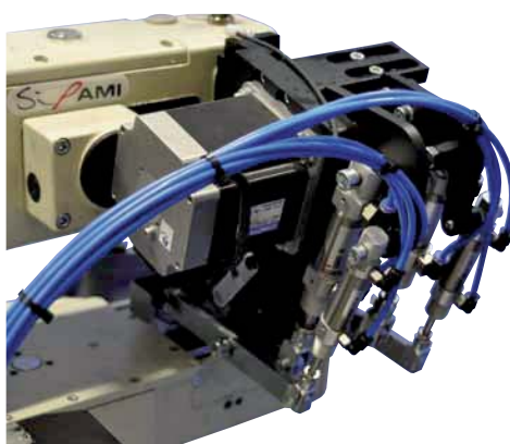
Electronic puller device
